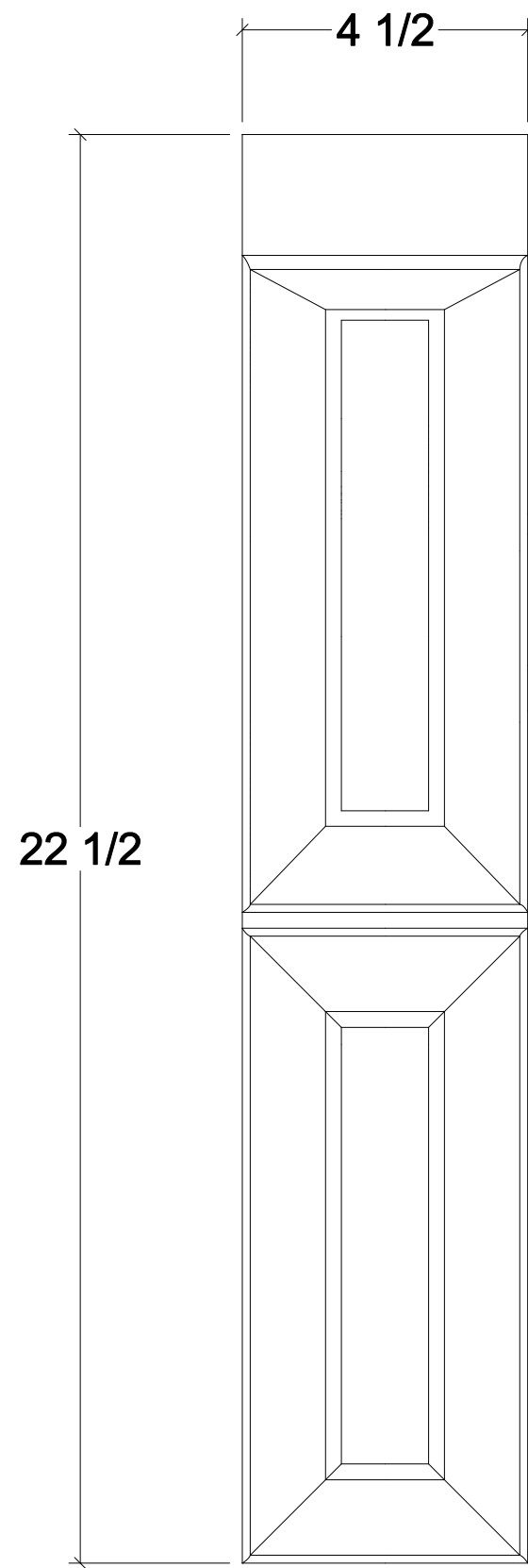
Front view
